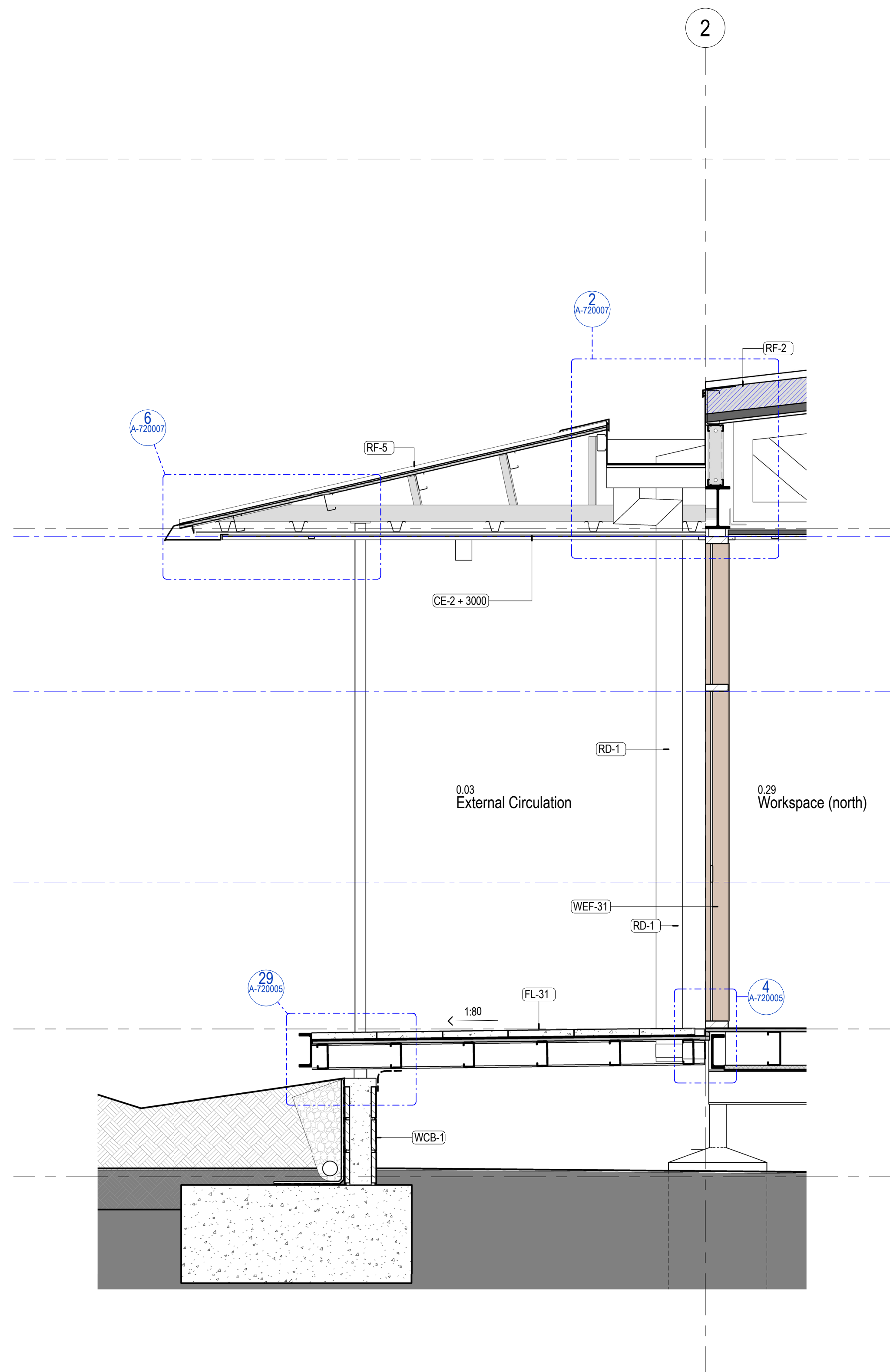
2 Courtyard North + West Facade Section 1 : 20
